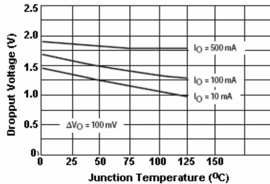
FIGURE 4 - Dropout Voltage v.s. Junction Temperature
