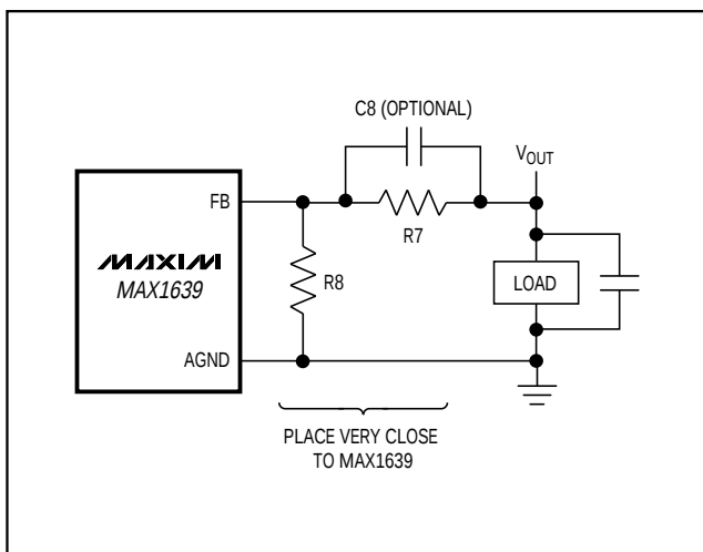
Figure 6. Output Selection
