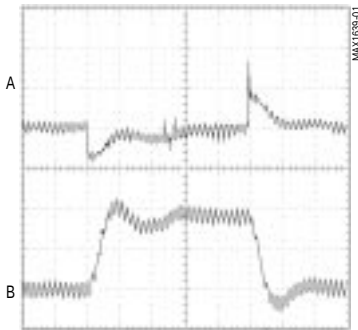
LOAD-TRANSIENT RESPONSE (V OUT = 2.5V)
