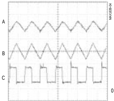
SWITCHING WAVEFORMS
