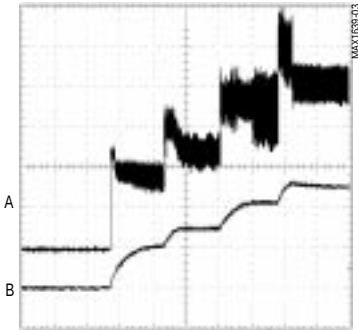
START-UP WAVEFORMS
