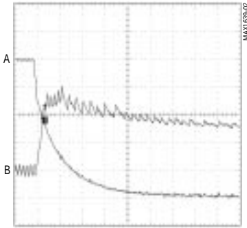
FOLDBACK CURRENT LIMIT (V OUT = 2.5V, NOMINAL)
