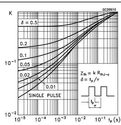
Figure 2. Thermal impedance for TO-220/ D 2 PAK
